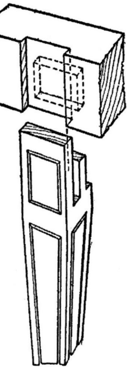
Fig. 141. — Method of Fitting an In- terior Table Leg.
