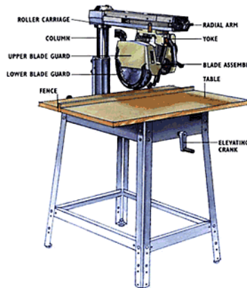
wood working power tools
