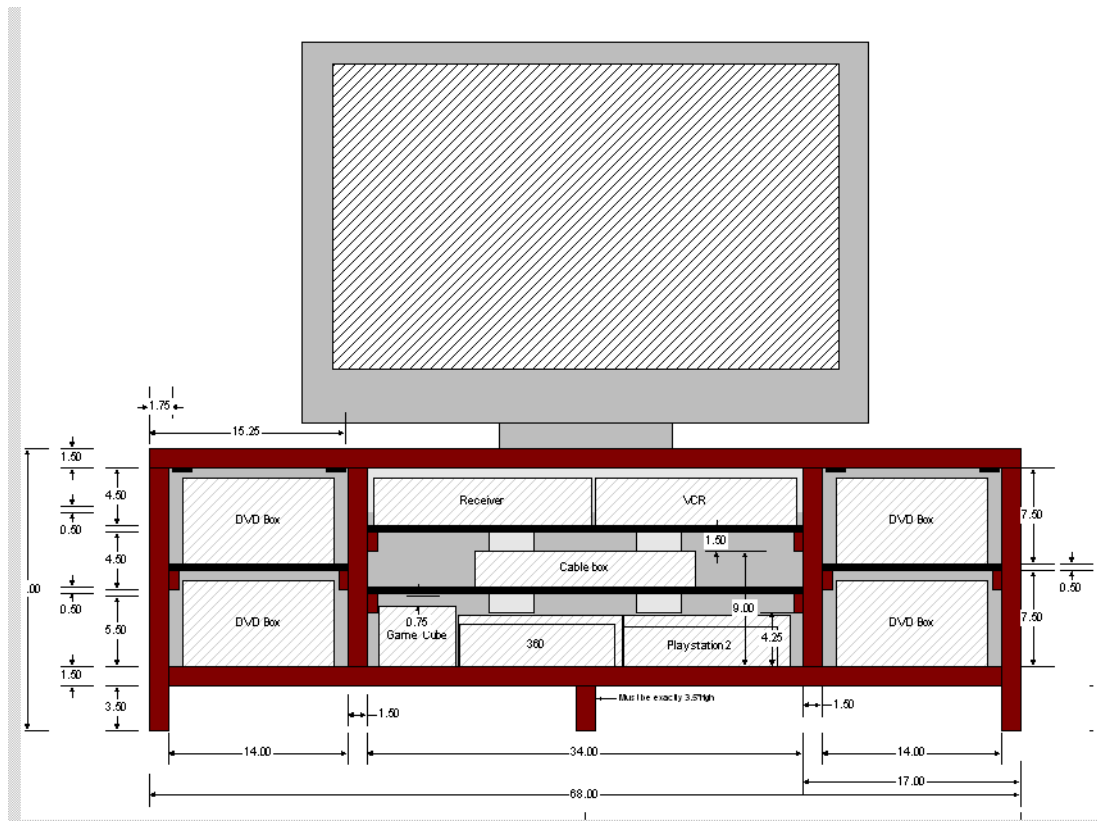
wood tv stand plans
