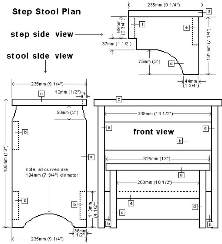
wood stool plans
