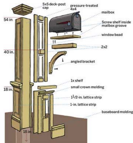
wood mailbox post plans
