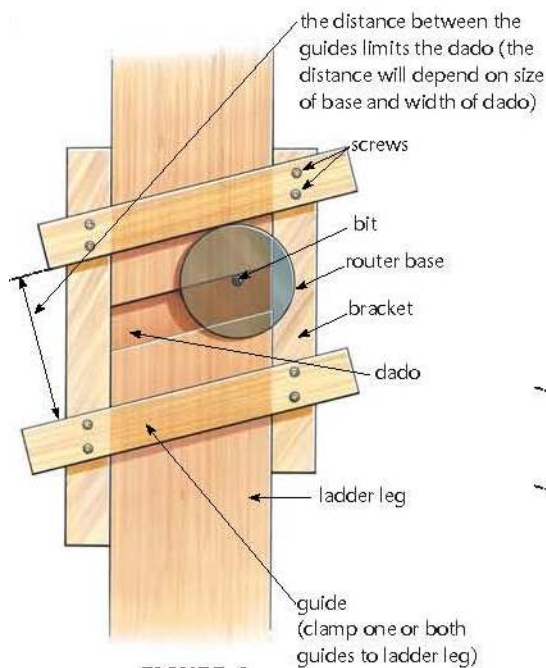
FIGURE 4 Jig to cut ladder-rung dados
