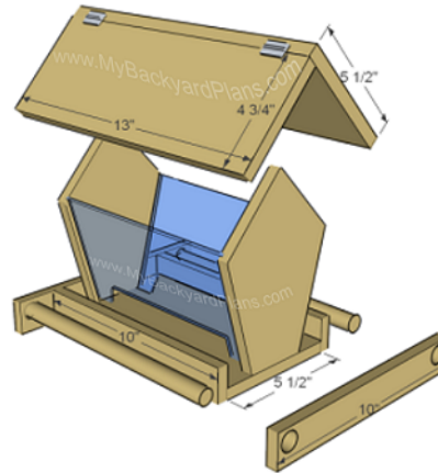
wood bird feeder plans
