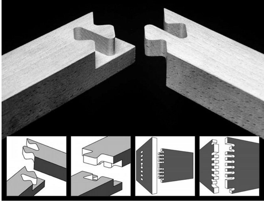
Japanese Woodworking Joints
