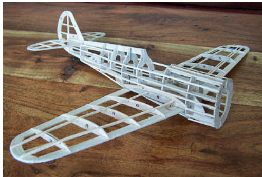
balsa wood glider plans
